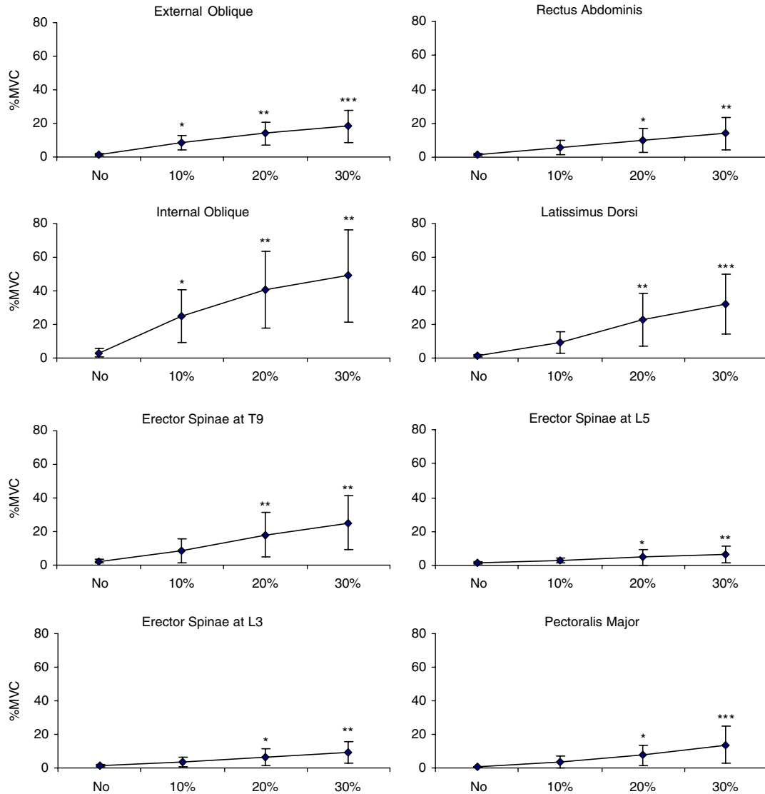
Fig. 3. Averages and standard deviations of the normalized EMG amplitudes before the perturbation for the right side muscles and four preactivation levels (no brace, 10%, 20% and 30% MVC). While the external oblique muscle was monitored for subject feedback, the internal oblique channel responded with higher activation levels and rectus abdominis with lower than target levels of activation. Results of the multiple comparison ( P < 0.05 ): *significantly higher than no brace; **significantly higher than no brace and 10% MVC; ***significantly higher than no brace and 10% and 20% MVC.
