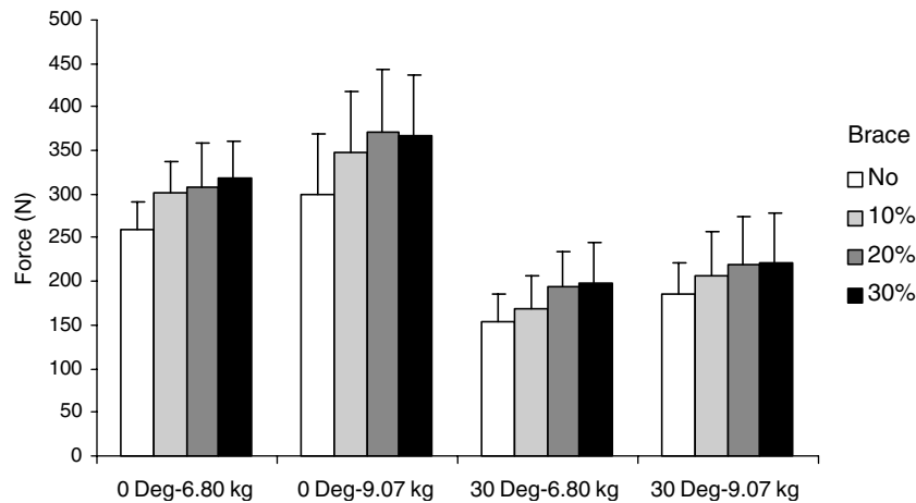
Fig. 5. Averages and standard deviations of the peak force magnitudes during the perturbation for two loading directions, two loading amplitudes, and four preactivation levels. The increasing coactivation levels stiffened the torso, reducing the trunk “shock absorption”, and caused higher peak cable tensions to develop.
