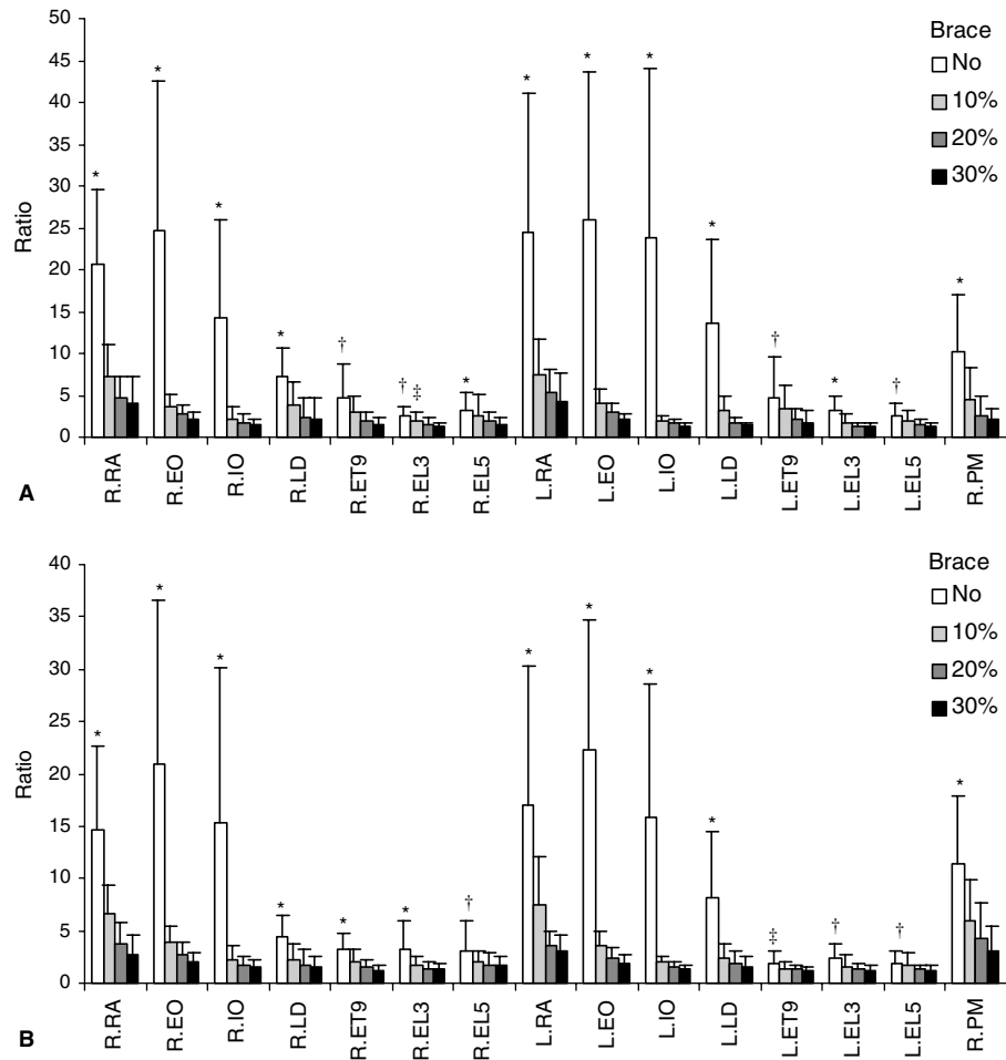
Fig. 8. Averages and standard deviations of the EMG response/preactivation ratios for four preactivation levels. (A) 0°-sagittal condition; (B) 30°-sagittal condition. The trunk preactivation increased the torso stiffness, thereby reducing the need for high muscle responses in order to stabilize the spine after sudden loading. Results of the multiple comparison ( P < 0.05 ): *significantly higher than 10%, 20% and 30% MVC; †significantly higher than 20% and 30% MVC; ‡significantly higher than 30% MVC.
