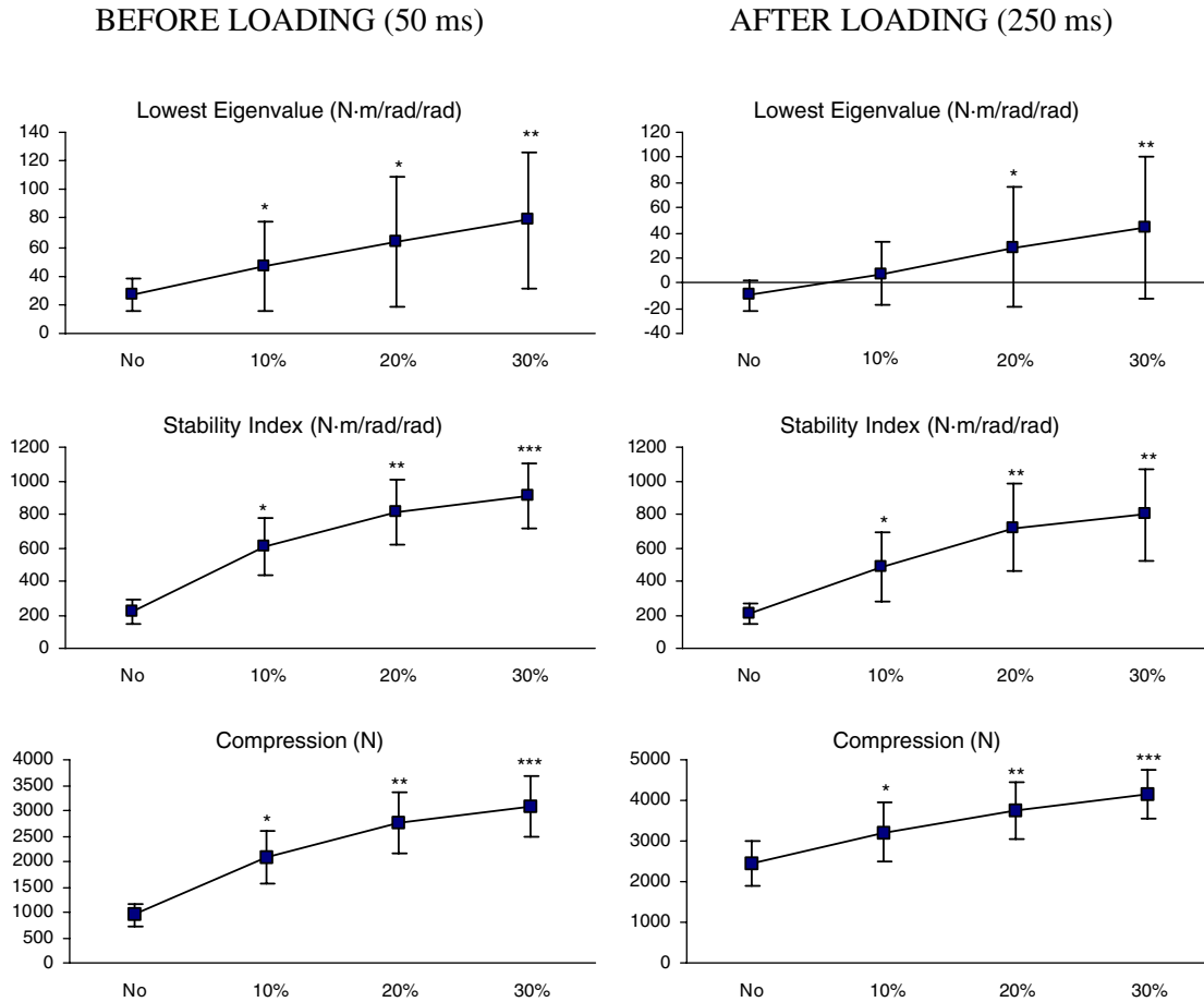
Fig. 4. Averages and standard deviations of the lowest eigenvalue, the stability index and the compression force for four preactivation levels (no brace, 10%, 20% and 30% MVC). This was examined both as the average over the 50 ms preload, and as the peak compressive force and minimum lowest eigenvalue and stability index post-load. More preactivation stiffens and stabilizes the spine at the cost of higher spine compressive load. Results of the multiple comparison ( P < 0.05 ): *significantly higher than no brace; **significantly higher than no brace and 10% MVC; ***significantly higher than no brace and 10% and 20% MVC. Note that possible instability occurred after loading with no brace as indicated with the negative value.
